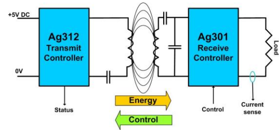
Ag300 Series Solution Tx/Rx overview
