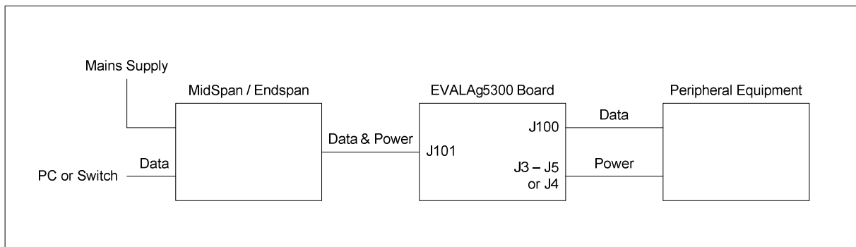
Figure 3: Example set-up
