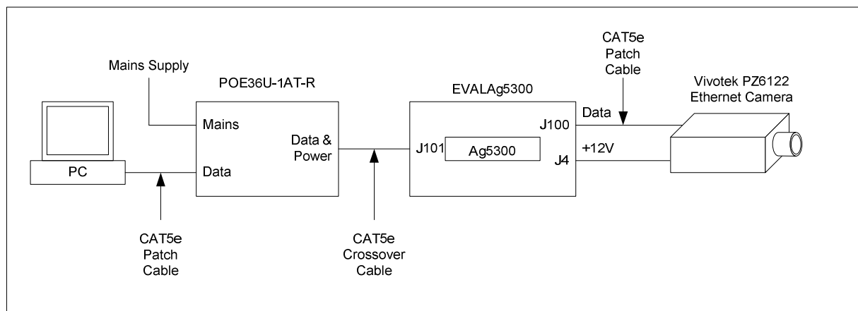
Figure 2: Basic set-up
