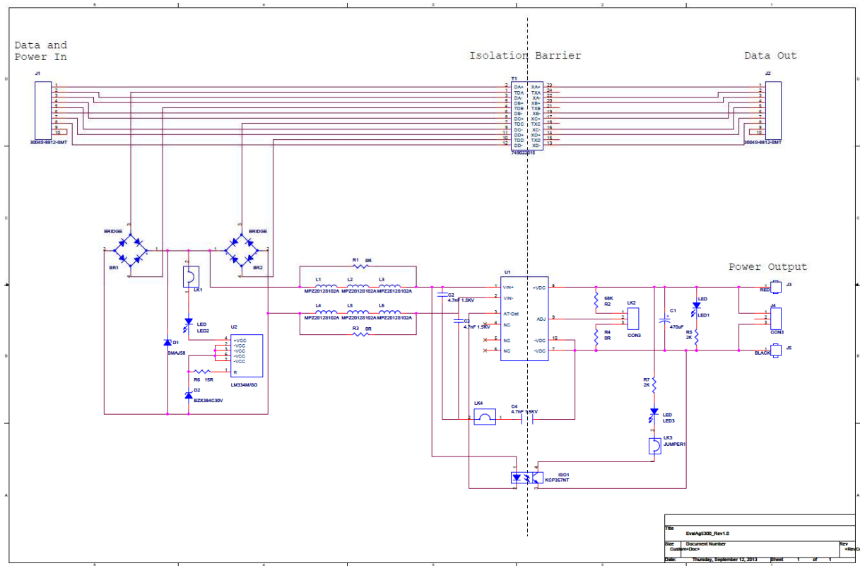
Figure 4: Board Schematic
