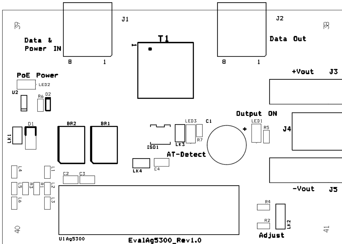
Figure 1: Board Layout
